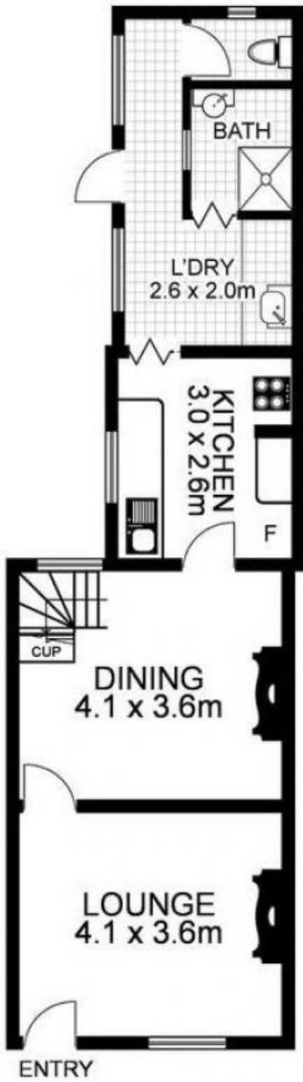
GROUND FLOOR
